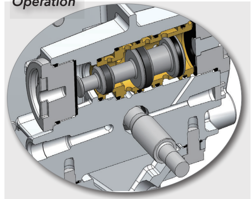
Stall-Free Operation
